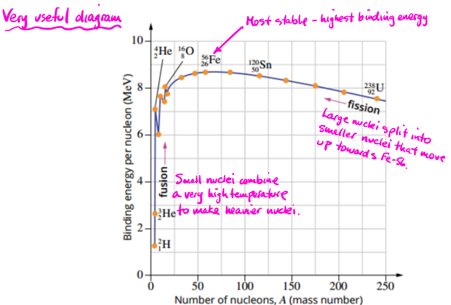
FIGURE 4.3.6 The graph of binding energy per nucleon.
